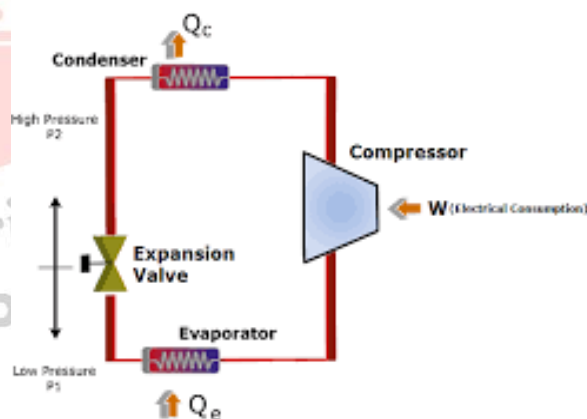
Fig1: VAPOUR COMPRESSION REFRIGERATION SYSTEM
